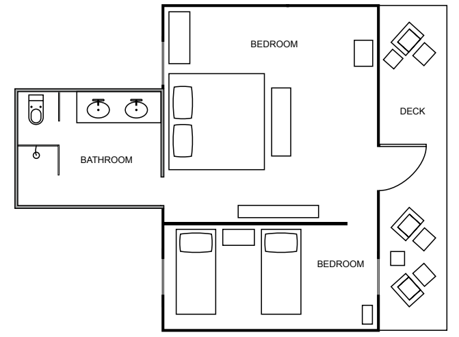
TWO-BEDROOM TENT WITH EN SUITE BATHROOM 975 SQUARE FEET
